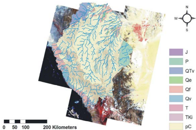
Fig 7: Geological features of the study area within the designated watershed.
