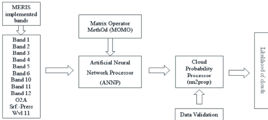
Fig 2: MERIS Cloud detection algorithm.
