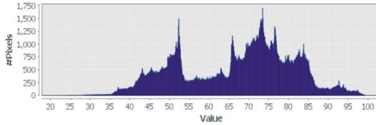
Fig 6: Relative humidity validation using cloudy mask.
