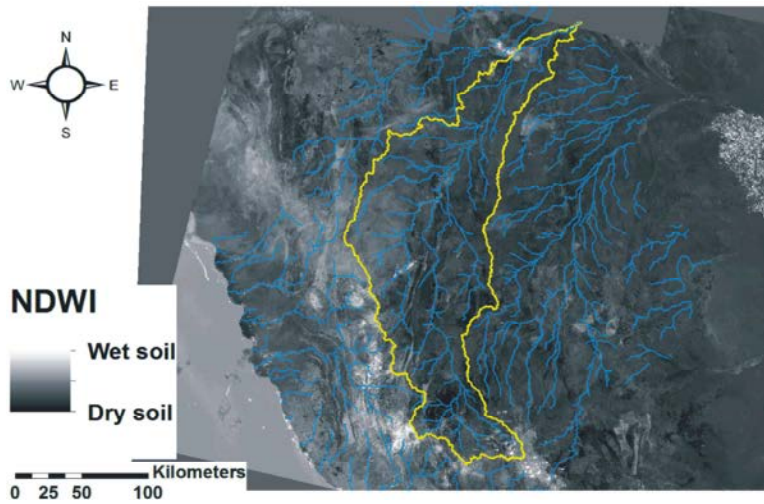
Fig 8: Normalized Difference Water Index map of the study area.
