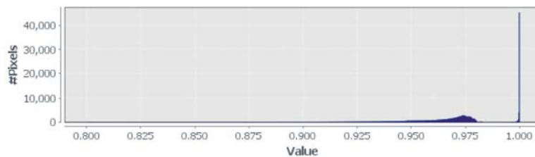
Fig 4: Stratocumulus clouds validation using cloudy mask
