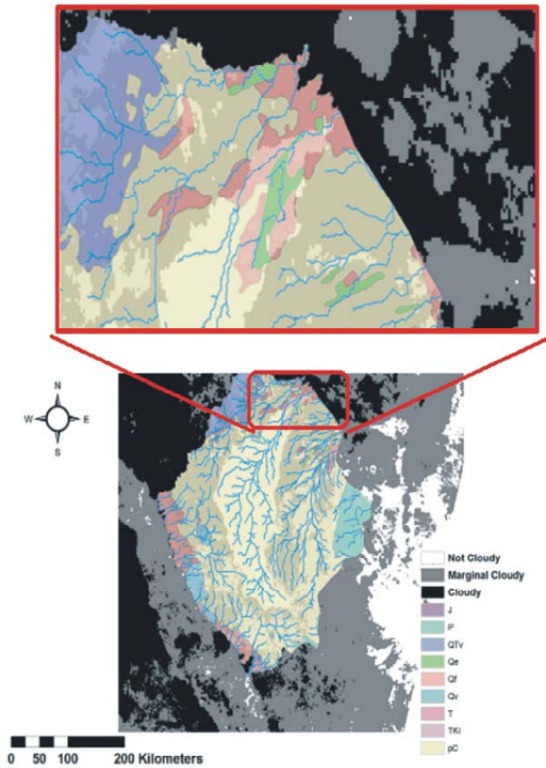
Fig 9: Suggested area for groundwater recharge improvements.
