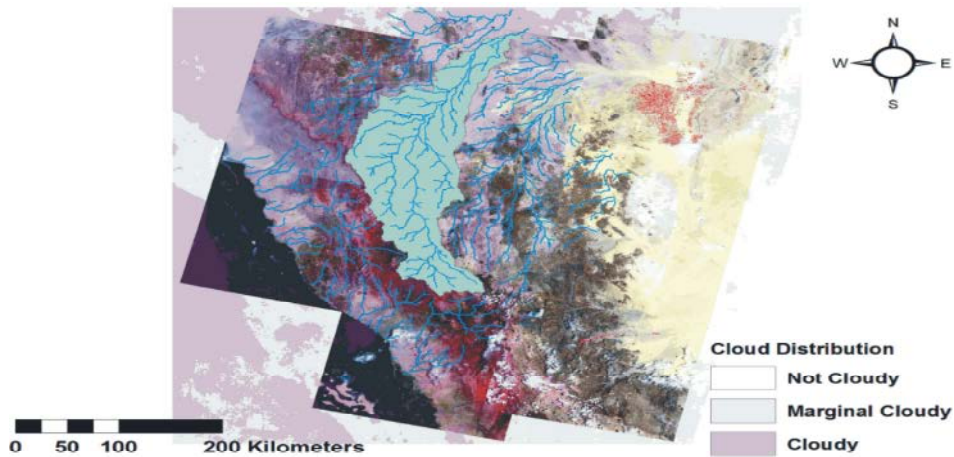
Fig 3: Study area in false color composition with cloud coverage classes.
