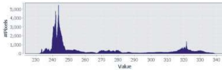
Fig 5: Total Ozone validation using cloudy mask
