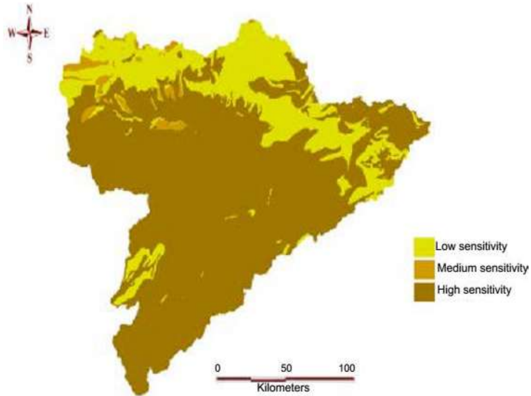
Fig. 3: Erosion sensibility of Ksob watershed versus the geology
