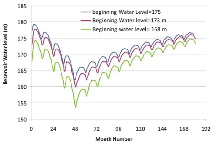
Fig. 4: Water level variation in Nasser Lake during and after filling period of GERD dam’s reservoir for impounding period of 3 years.
