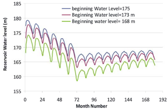
Fig. 6: Water level variation in Nasser lake during and after filling period of GERD dam’s reservoir for impounding period of 5 years with 0.5 BCM monthly reduction in discharge.
