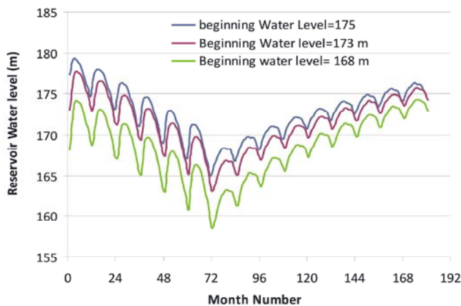
Fig. 5: Water level variation in Nasser lake during and after filling period of GERD dam’s reservoir for impounding period of 5 years.
