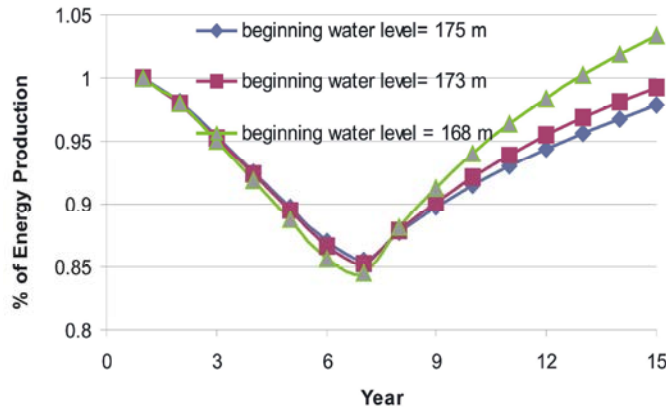
Fig. 8: Ratio of yearly energy production to the base year during and after GERD filling.
