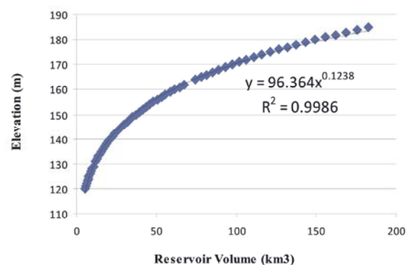
Fig. 2: Variation of water level in Nasser Lake with storage volume in the reservoir.
