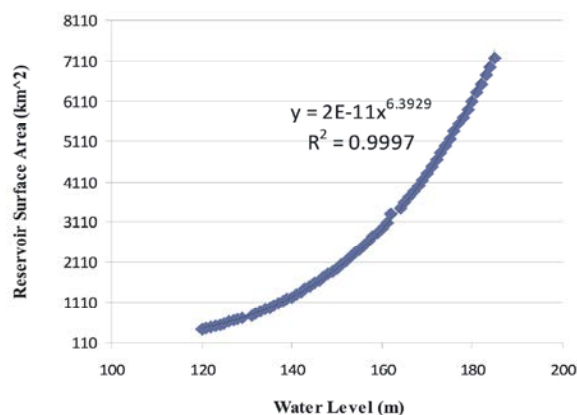
Fig. 1: Variation of Nasser Lake water surface area with water level in the reservoir.
