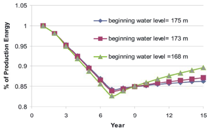
Fig. 9: Ratio of yearly energy production to the base year during and after GERD filling with reduction in inflow discharge.
