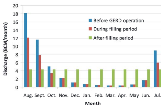
Fig. 3: Monthly Discharge at the mouth of Blue Nile before GERD operation, during filling period and after operation.
